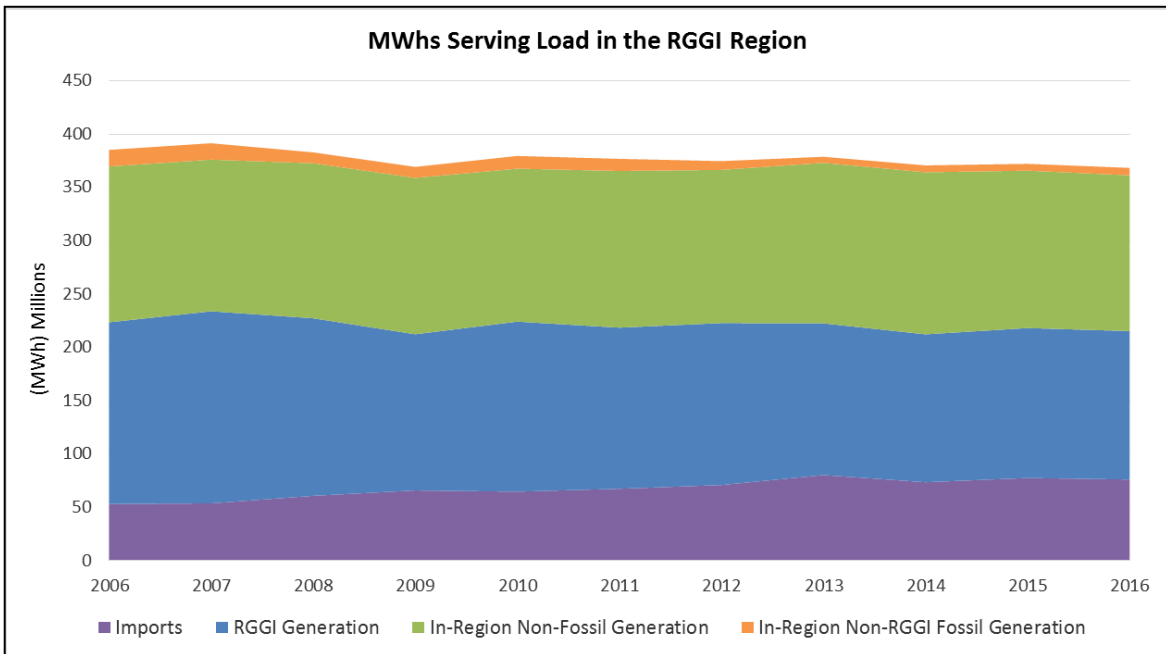
Figure 3. MWh of generation serving load in the RGGI region from 2006-2016.
