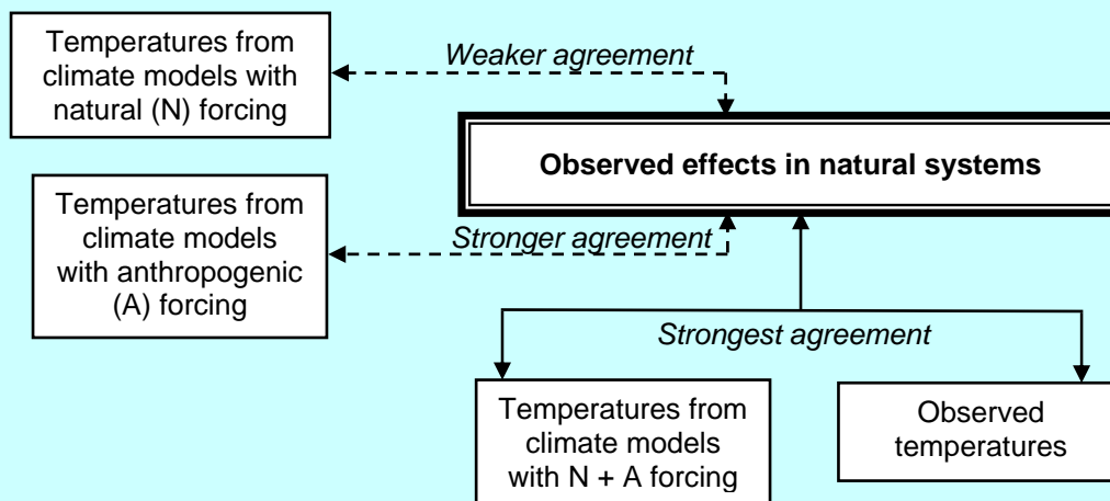
Box SPM-1. Linking the causes of climate change to observed effects in natural systems
