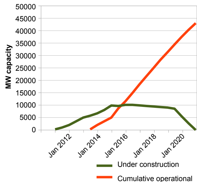
FIGURE 13 Solar Thermal Installation Timeline
