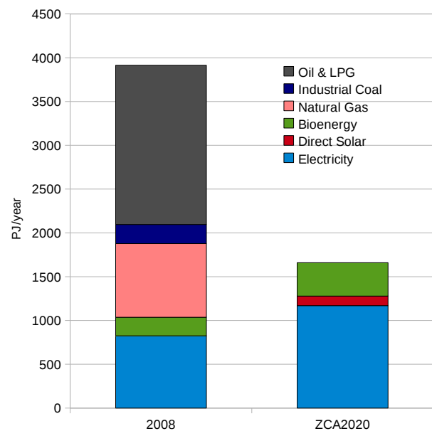
FIGURE 3 Australian Energy Sources: Present and Under ZCA2020
