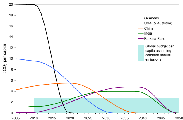
FIGURE 2 Global Carbon Budget for Emissions
