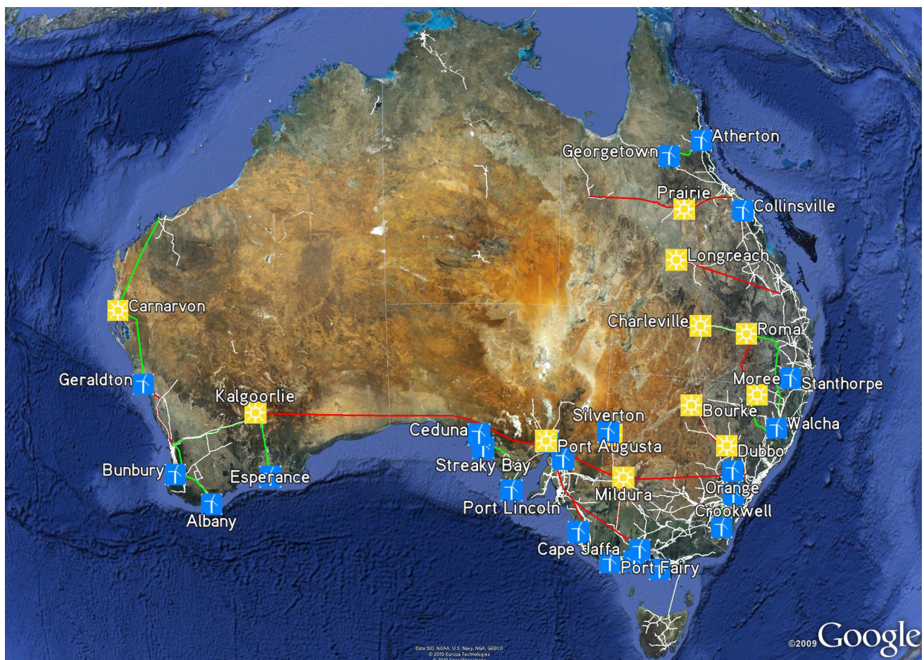
FIGURE 6 ZCA2020 Proposed 100% Renewable Grid
